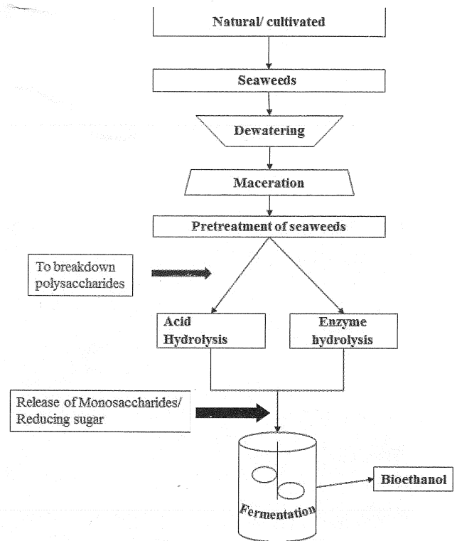
Figure 1 : Schematic representation of bioethanol production from macro algae or seaweed
